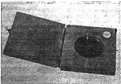
Figure 1 Spherical densimeter, Model A, with estimating grid scratched on the surface of the convex mirror
